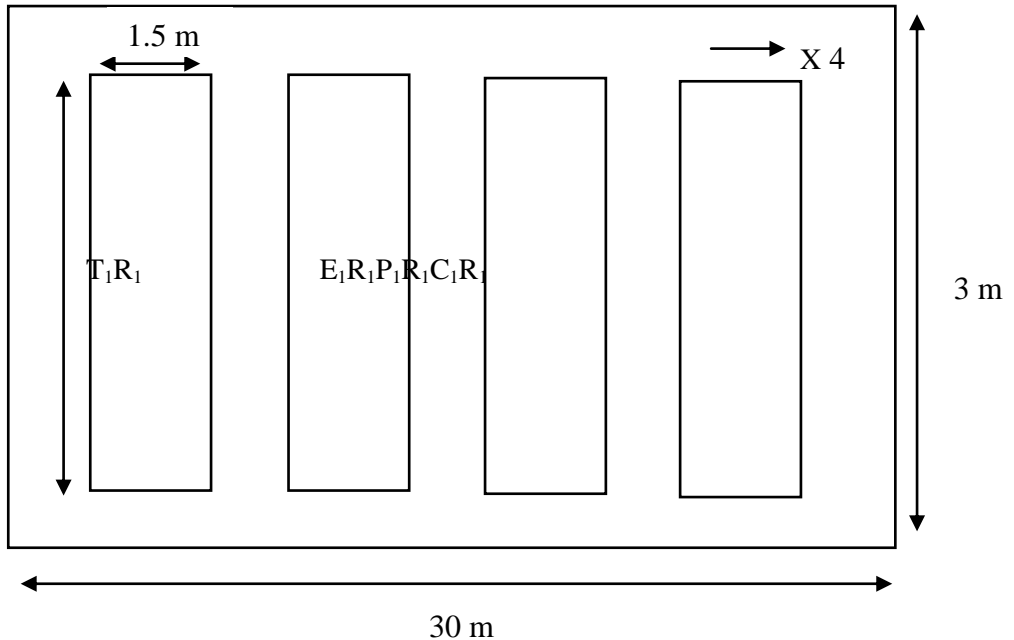
Figure 01: Detailed experimental layout for soil erosion measurements
