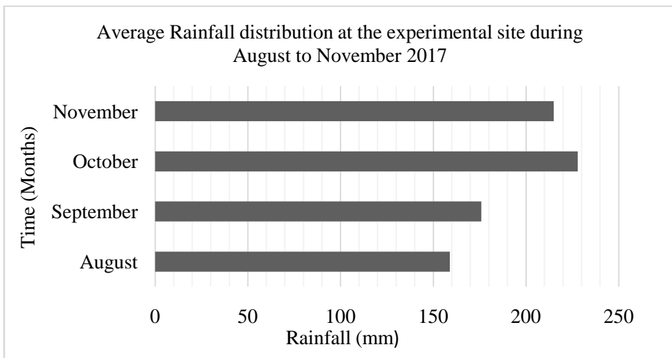
Figure 2: Average Rainfall distribution at the experimental site during August to November 2017
